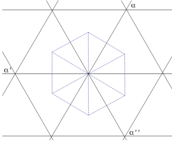
FIGURE 3. The inner hexagon with dashed lines, which equals \text{conv}(W_\Phi) , is a fundamental domain for the regular triangles lattice generated by \Phi = \{\alpha, \alpha', \alpha''\} . The six points W_\Phi are its vertices.
