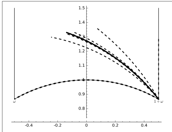
FIGURE 1. The dashed curves are cluster points of Dirichlet shapes of rings of the form \mathbb{Z}[\theta] where \theta is a unit, which we construct. The thick curve in the middle is (one of the countably many) limits of the dashed curves.
