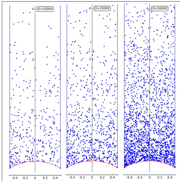
FIGURE 2. Above are sage plots of Dirichlet shapes of the unit lattices of rings of integers of totally real fields with discriminant bounded from above by 10000, 20000, 50000 respectively.
